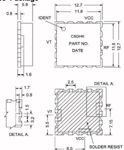
SK605 Package
